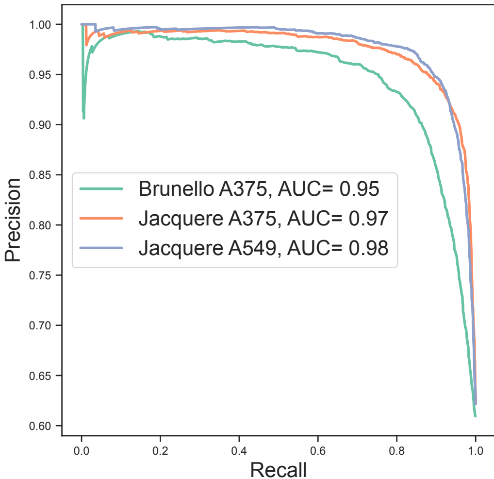
Jacquere split vector screen Precision Recall Curve
